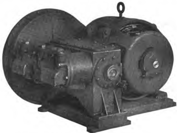
Fig. 4666. 14-H. P. Motor-Driven Air Compressor with 690-Volt A. C. Series Motor. Westinghouse A. C. Electric Locomotive.
